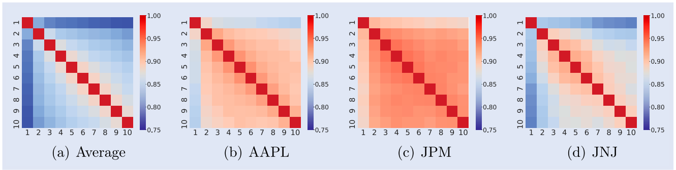
Figure 1. Correlation matrix of multi-level OFIs. (a) Average. (b) AAPL. (c) JPM and (d) JNJ.
